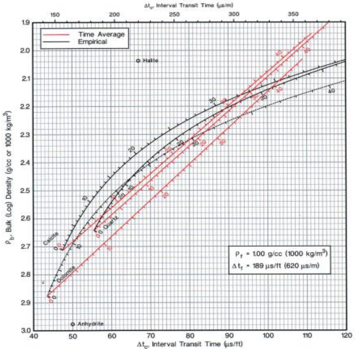
Sonic-density crossplot
