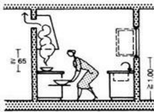
③ Low-level oven requires adequate space in front; extractor hood above cooker
