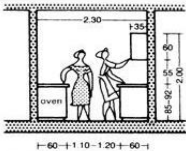
② Section through kitchen; space for two people
