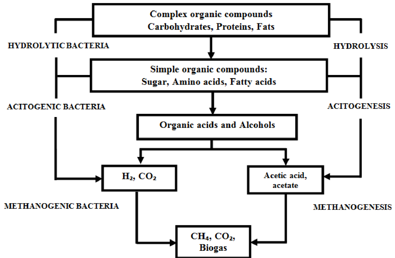
Fig 5. Flow chart showing the four phases of kitchen waste digestion
