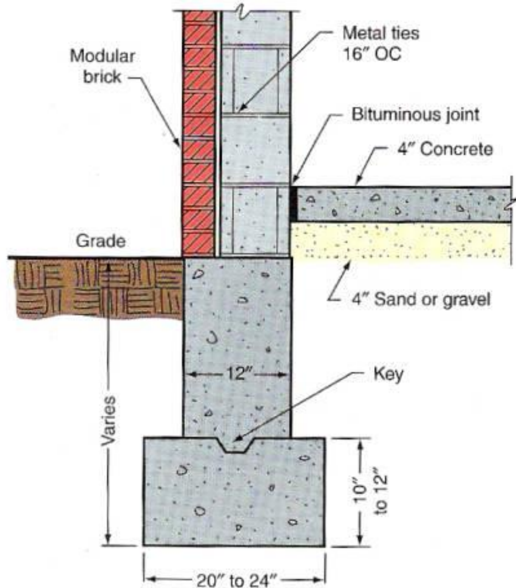
Poured concrete foundation for composite brick and block wall
